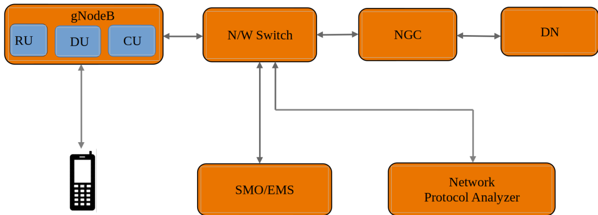
TEST SETUP 7
