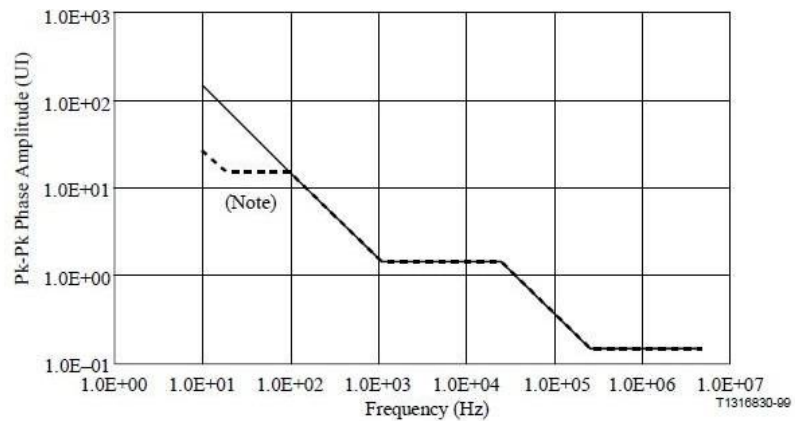
Figure 3/G.825
