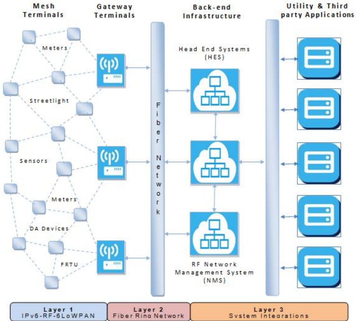
Fig ANNEX7.1: AMI Architecture with 6LoWPAN
