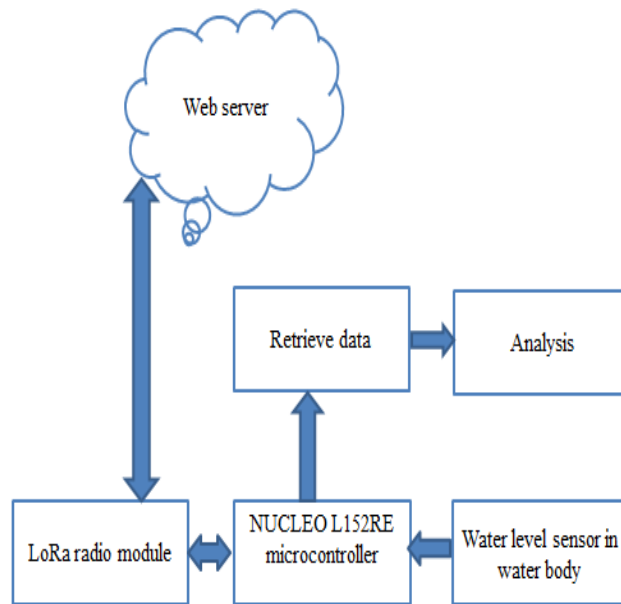
Fig ANNEX3.2: Block diagram of the proposed model
