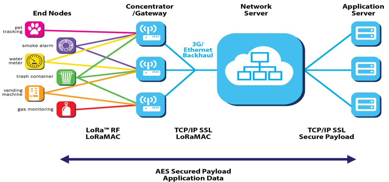
Figure 17 : LoRAWAN Protocol
