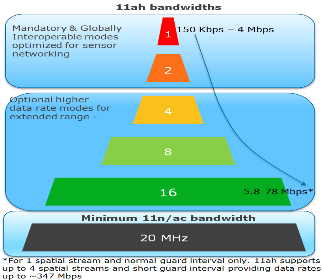
Figure 14 : 802.11ah Bandwidth Modes [11]
