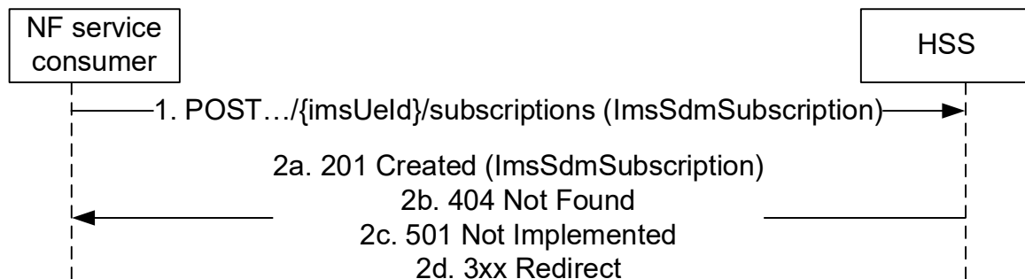
Figure 5.3.2.3.2-1: NF service consumer subscribes to notifications
